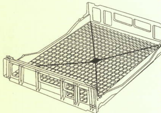
Bread tray (two ways) 26" x 24" x 6.5" No. 60313
